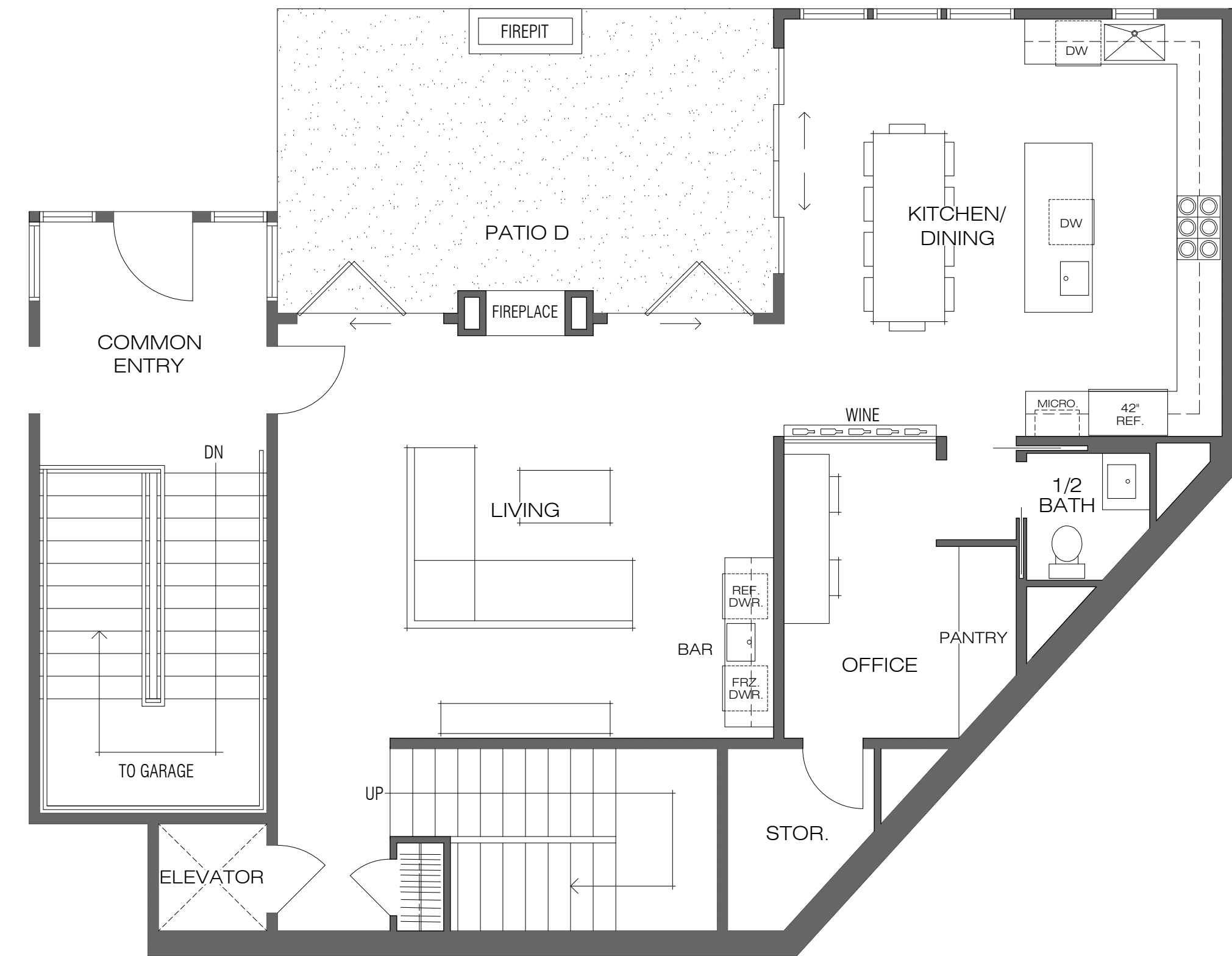
UNIT D TERRACE LEVEL FLOOR PLAN
