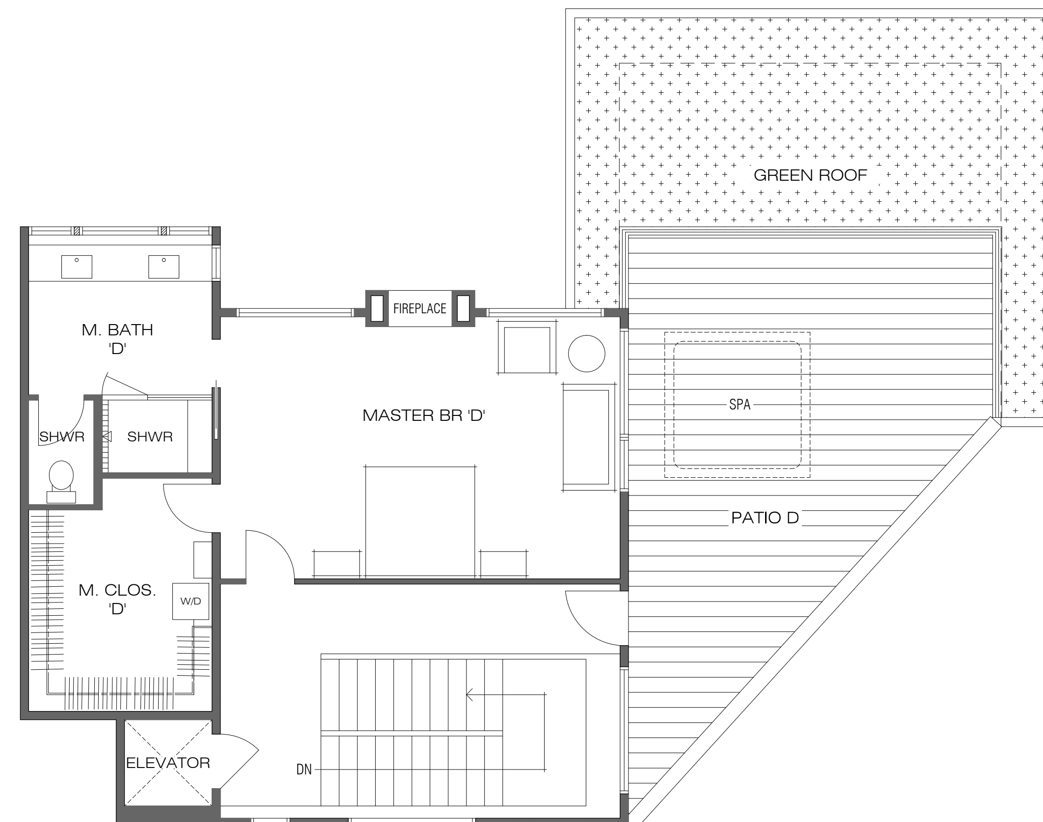
UNIT D MASTER LEVEL FLOOR PLAN
