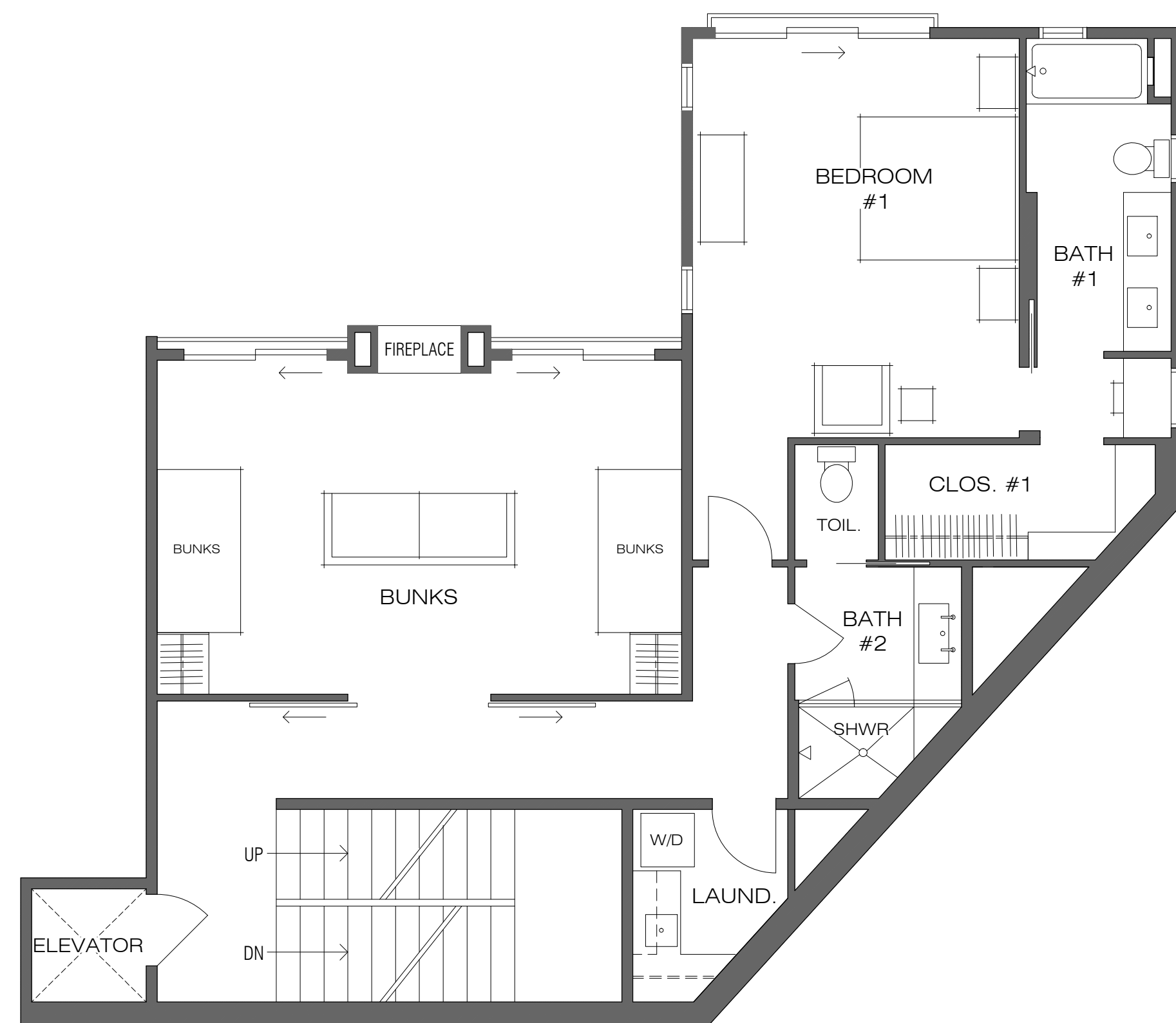
UNIT D SECOND LEVEL FLOOR PLAN
