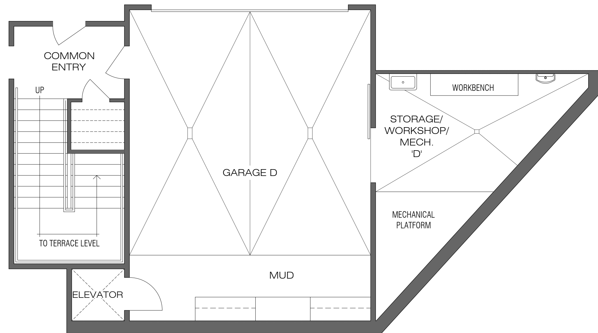
UNIT D GARAGE LEVEL FLOOR PLAN
