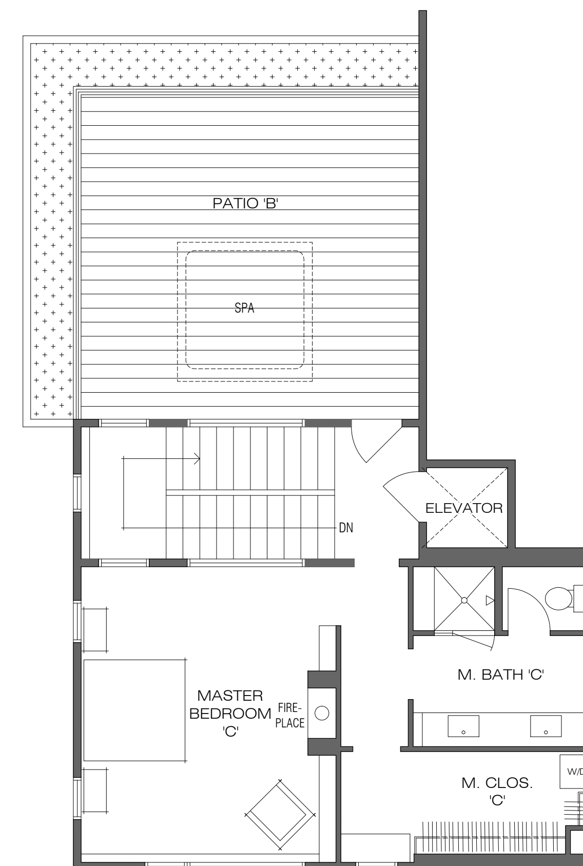
UNIT C MASTER LEVEL FLOOR PLAN
