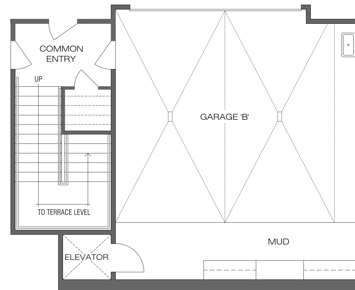
UNIT B GARAGE LEVEL FLOOR PLAN
