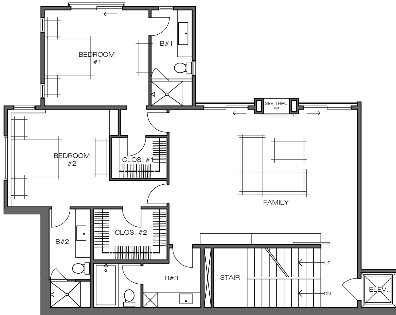
UNIT A SECOND LEVEL FLOOR PLAN
